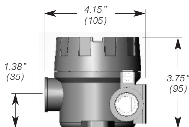
Aluminum Housing (XD)
