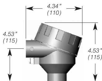
Aluminum Housing (AD)
