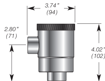
Stainless Steel Housing (SS)
