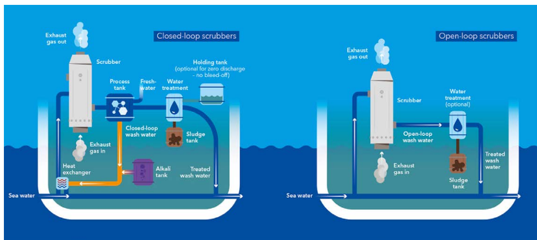
Main types of wet scrubber
