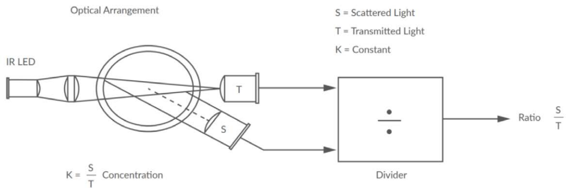
Diagram showing scattered light optical arrangement
