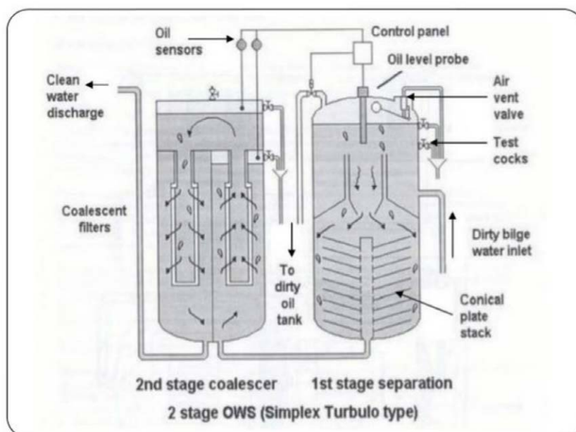
Gravity separation system
