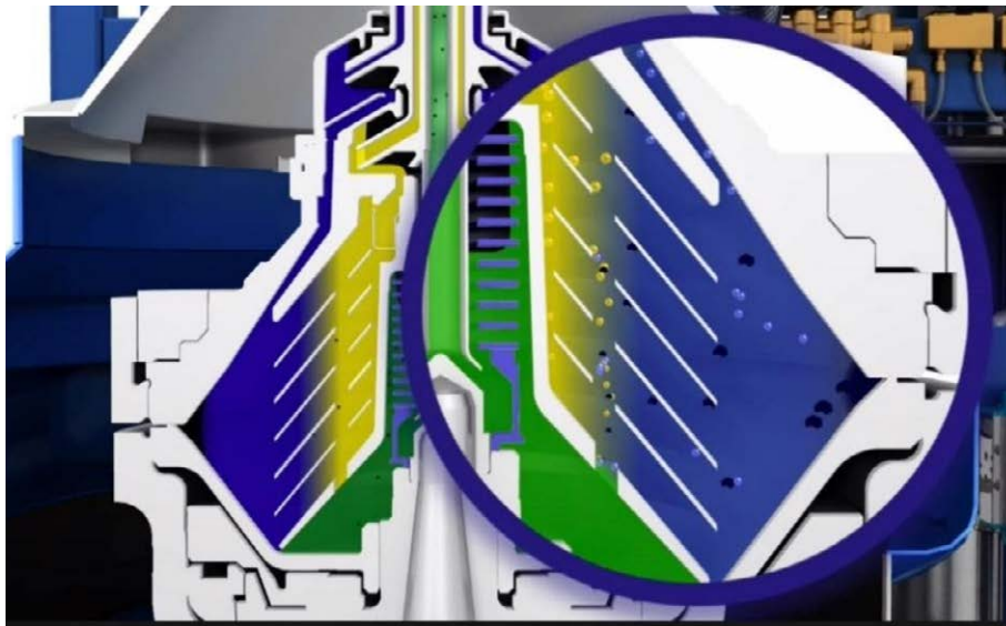
Centrifugal separation in Alfa Laval PureBilge
