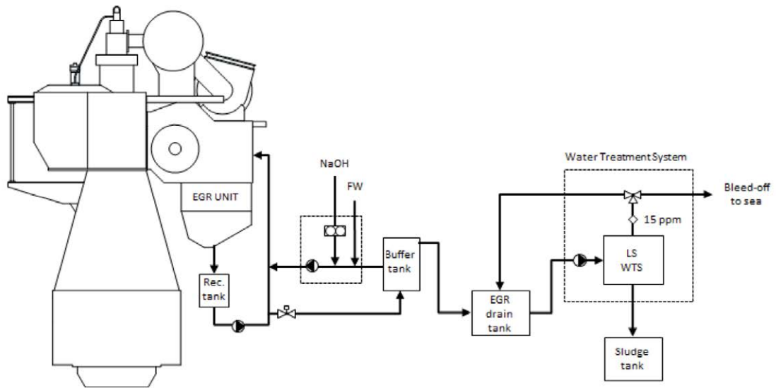
MAN ES Low Sulphur water handling
