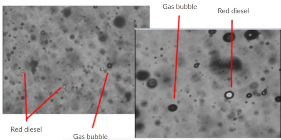
Diagram showing example images from microscopy camera
