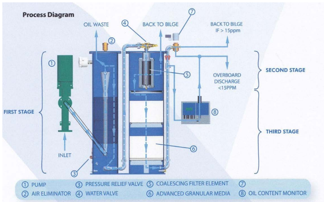
Adsorption – Victor Marine Separator
