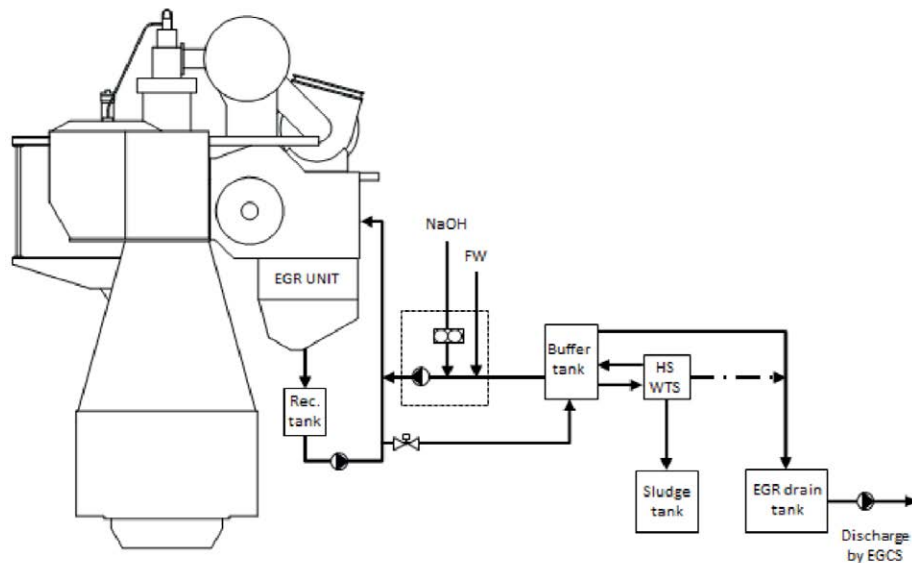
MAN ES High Sulphur water handling
